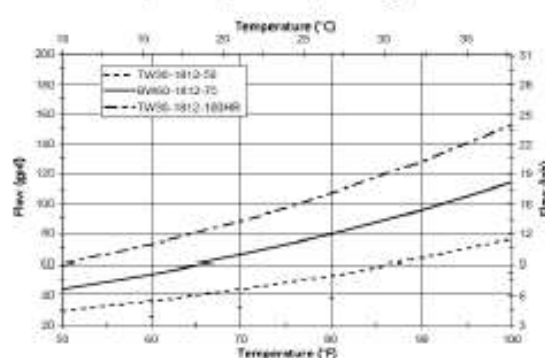
Figure 2: Impact of temperature on permeate flow (constant pressure, recovery)
